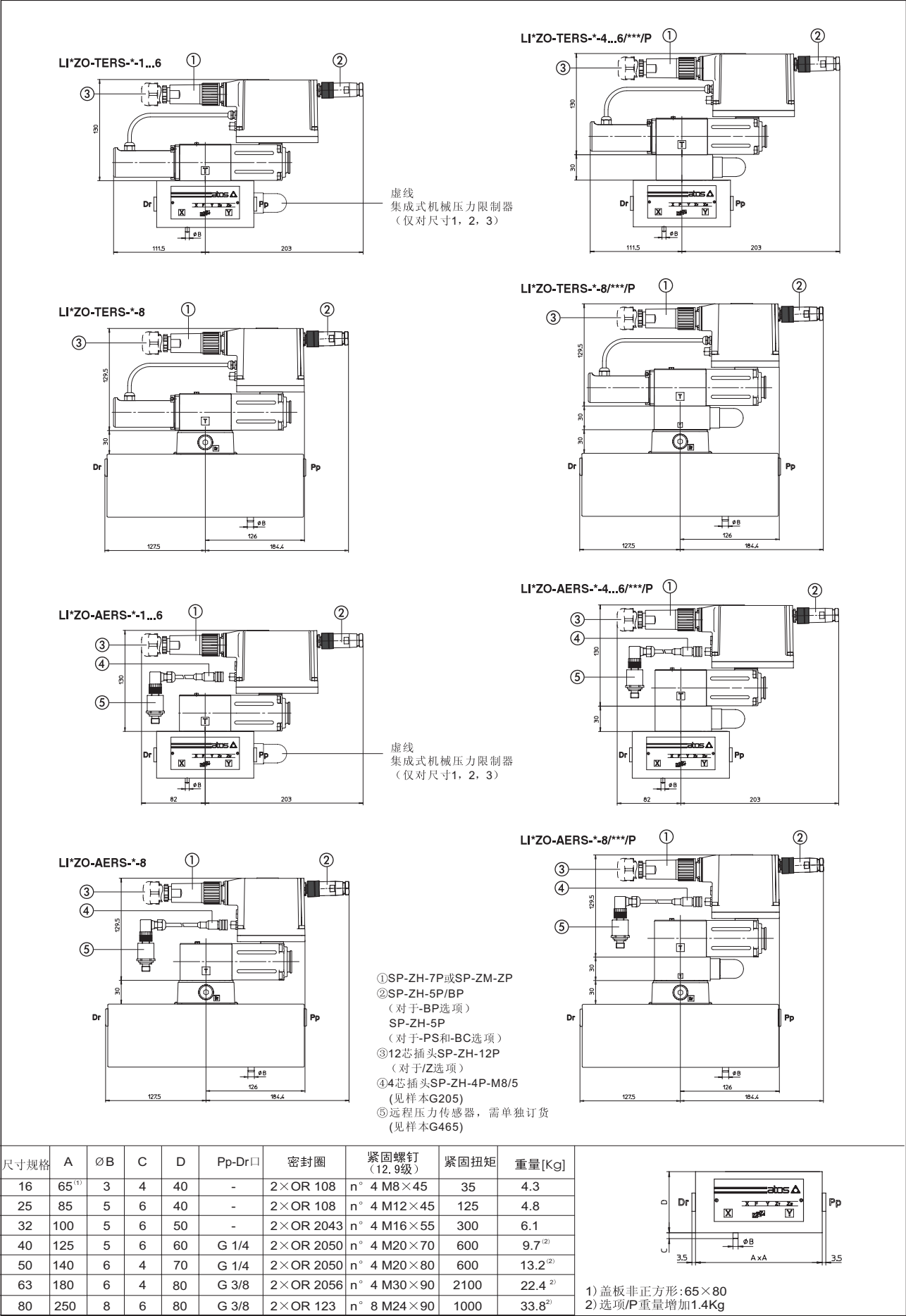
13 LI*ZO-TERS和-AERS的盖板尺寸 [mm]
